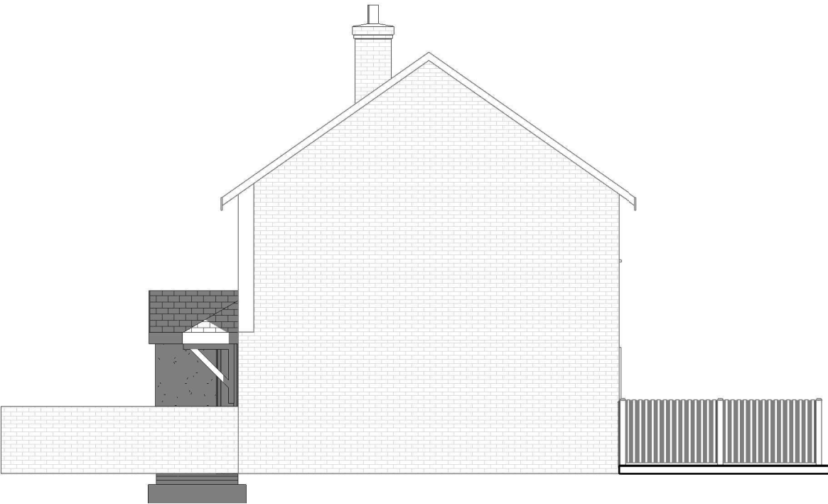
Proposed Elevation-Right side
