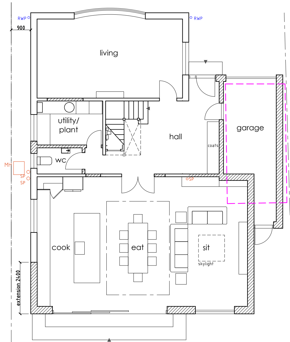
GROUND: PROPOSED 1:100
