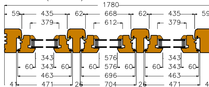
Section C2 (scale 1:5)
