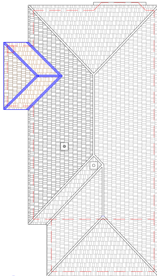
2 PROPOSED ROOF ELEVATION 1:100
