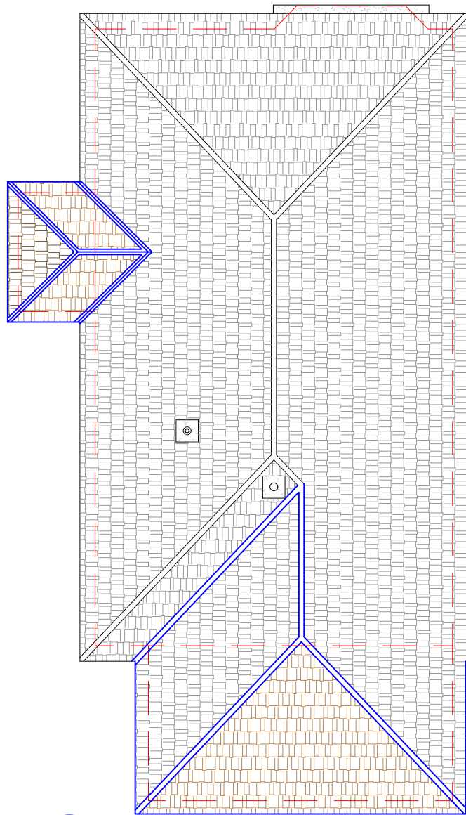
1 EXISTING ROOF ELEVATION 1:100
