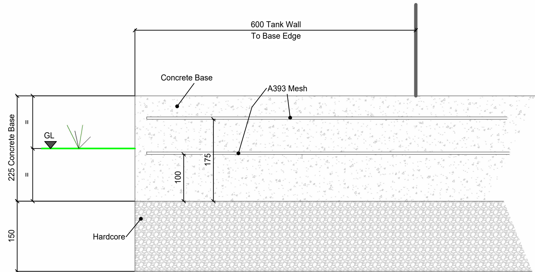
4 Hay, Storage Tank Base Section 1 : 5
