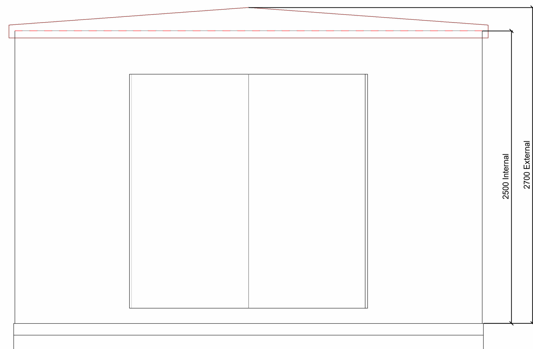
2 Hay, Pump House Elevation 1 : 20
