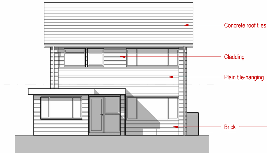
South Elevation - Existing-
