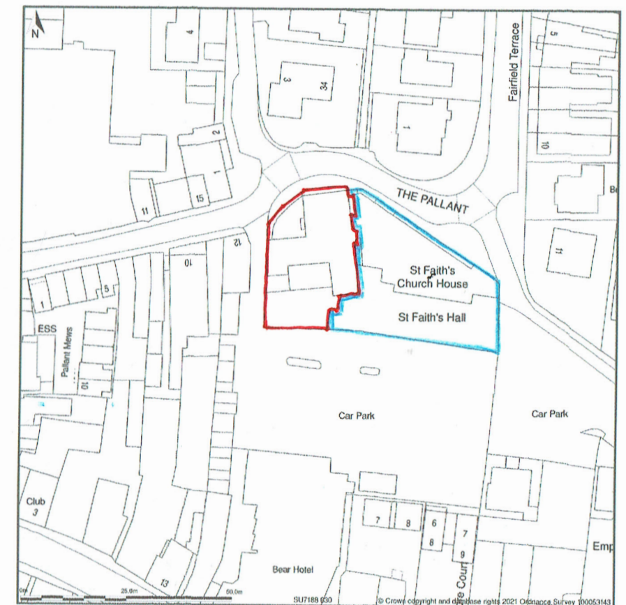
LOCATION PLAN 1:1250
